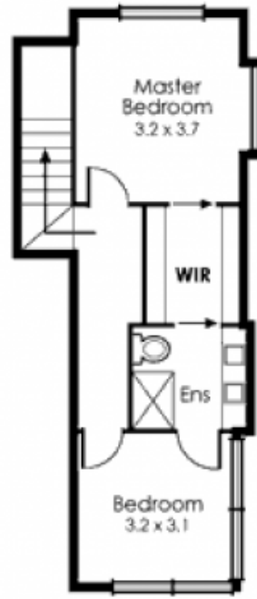
Top Floor
